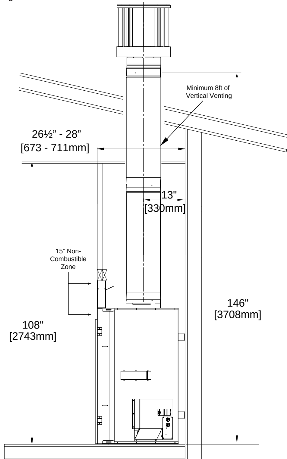
Figure 55: Minimum Vent for Propane [LP]
