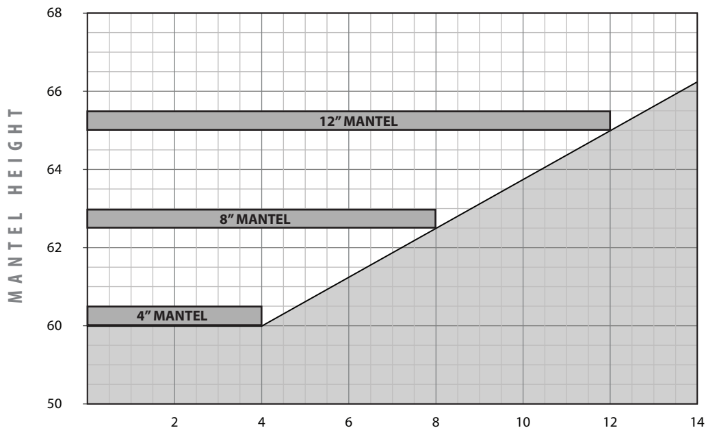
Figure 52: Mantel Clearances - Non CSS
