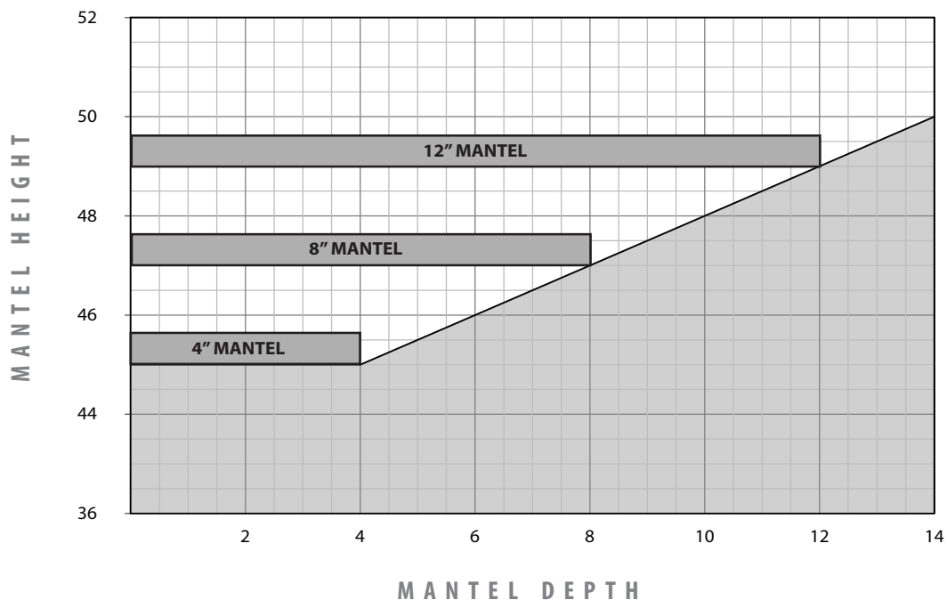
Figure 53: Mantel Clearances - CSS Activated
