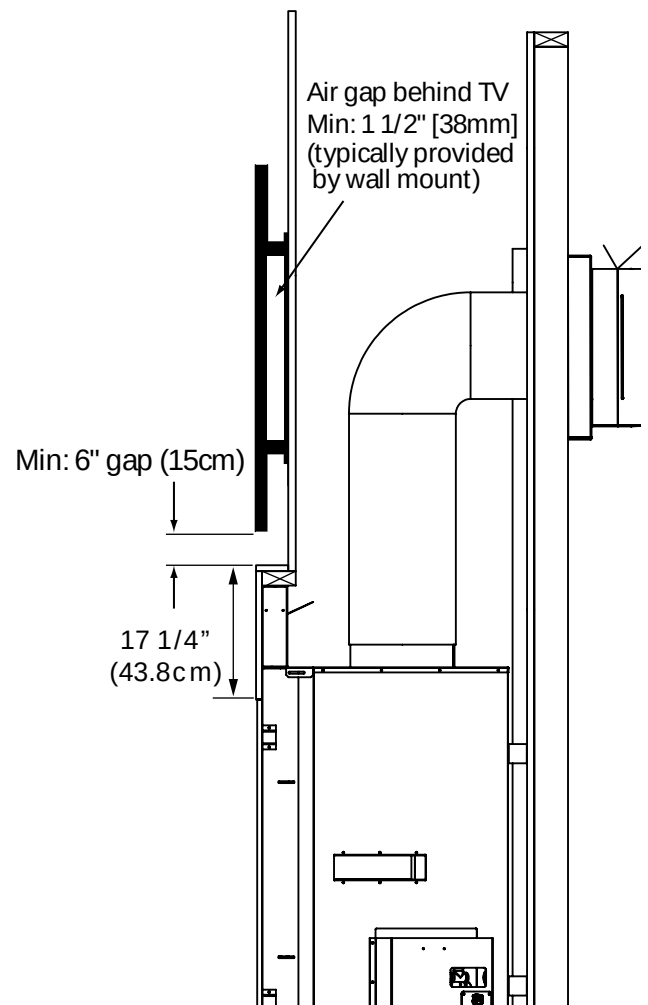
Figure 58: Recess Minimum TV Install
