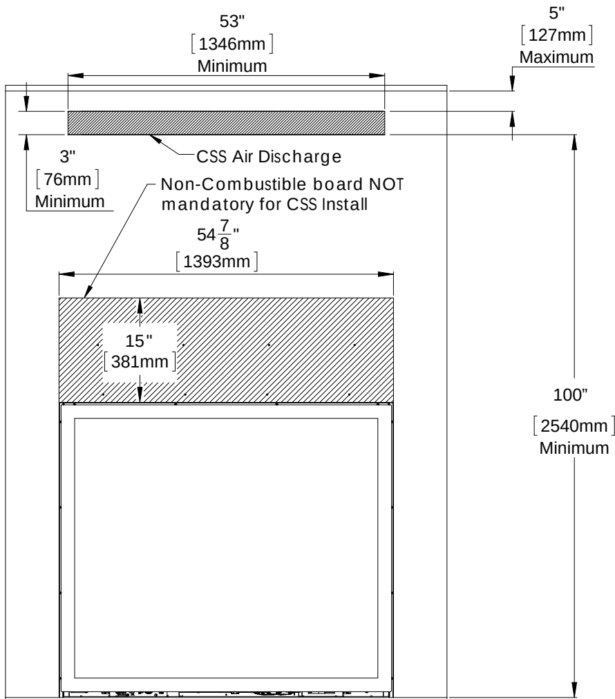
Figure 41: Framing Option 1
