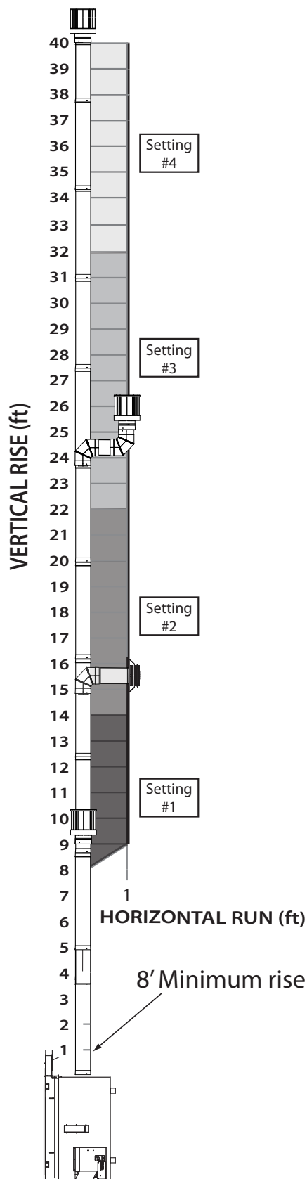
Figure 62: 8" x 11" LP Vent Graph
