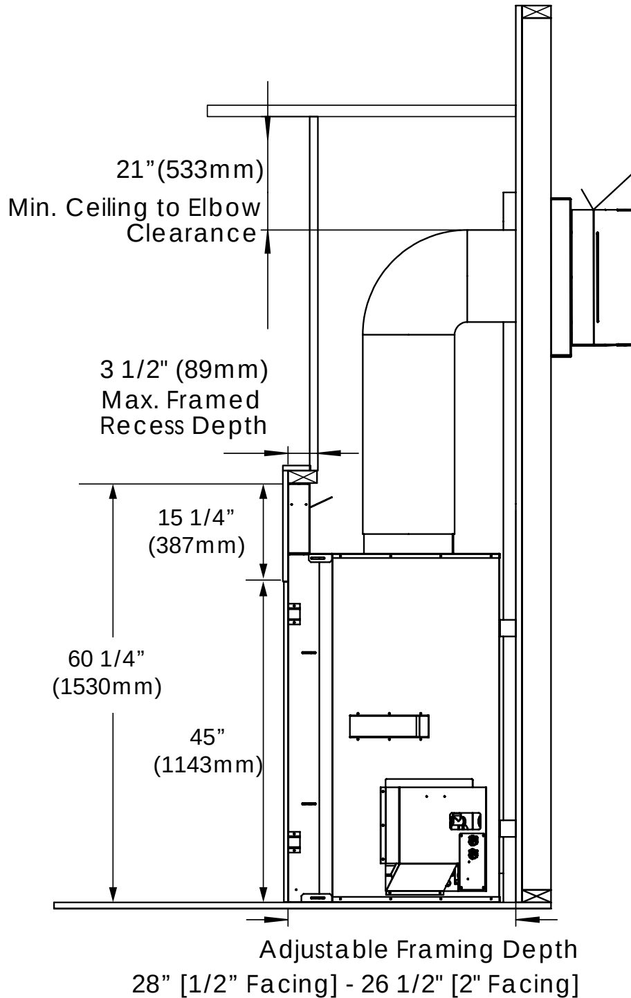
Figure 50: Recess Installation
