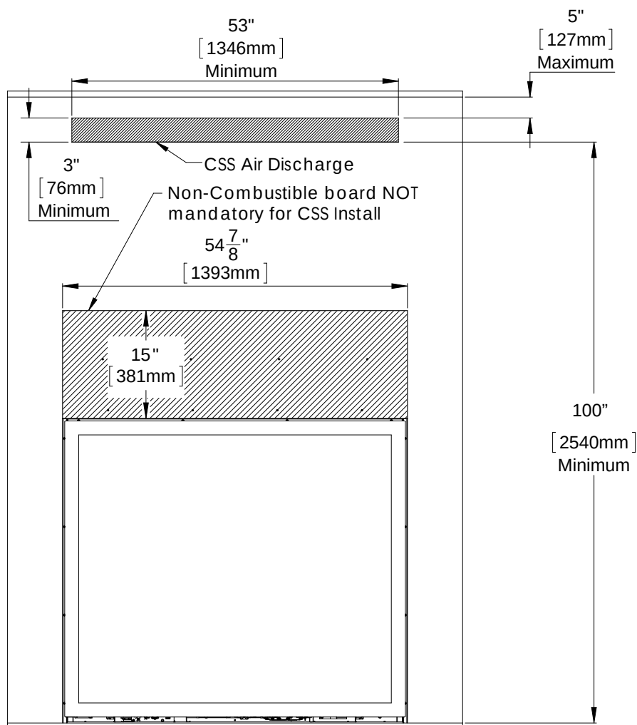
Figure 56: Typical Facing Layout
