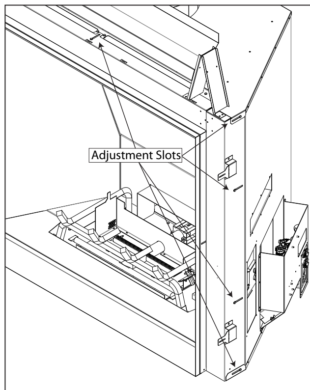
Figure 36: Framing Depth Adjustment
