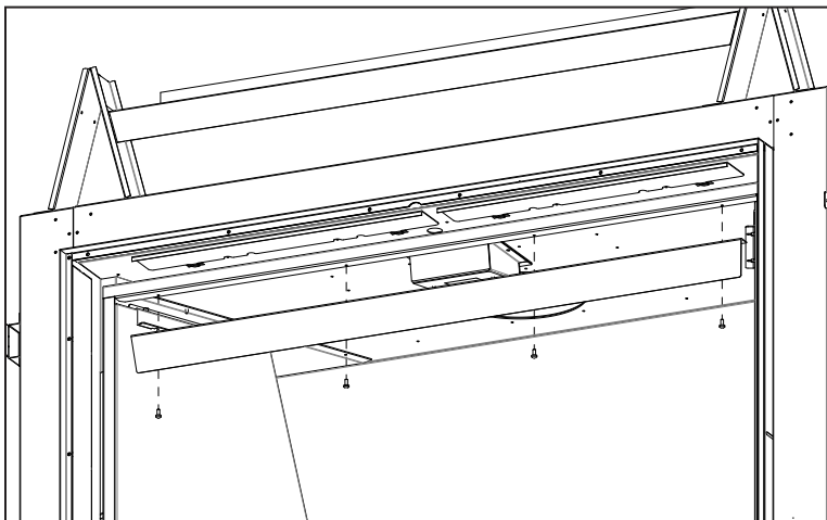
Figure 75: Light Deflector Removal
