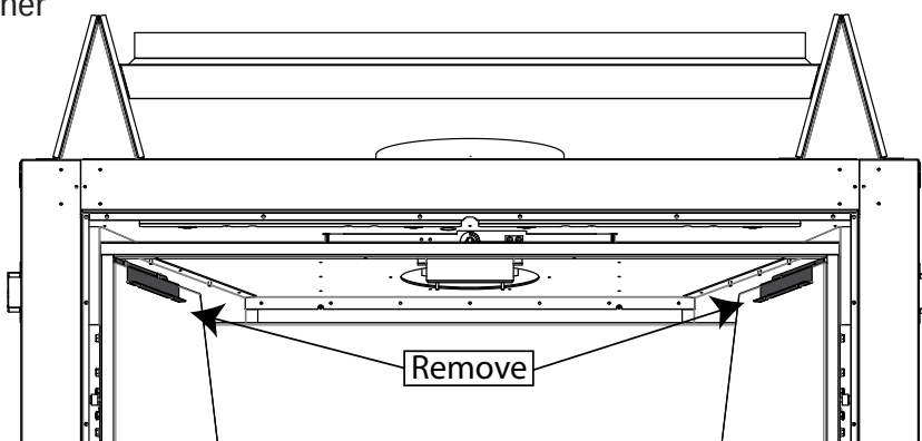
Figure 76: Liner Retainers
