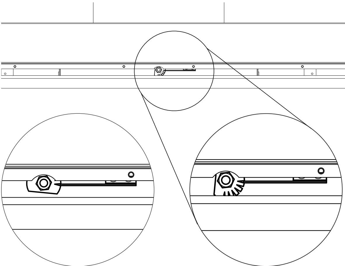
Figure 66: Restrictor Setting 6
