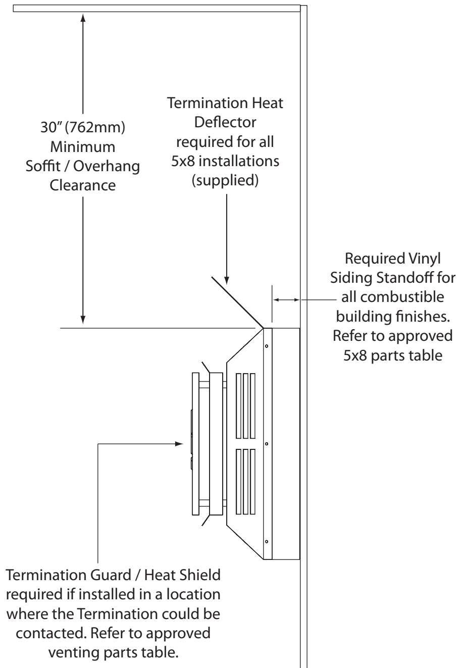
Figure 61: Additional Termination Restrictions for 5" x 8" Venting
