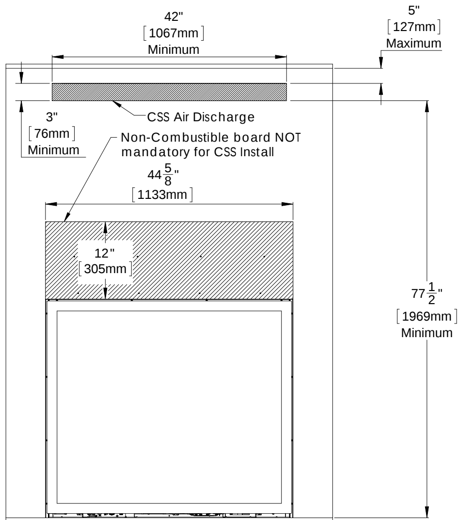
Figure 56: Typical Facing Layout
