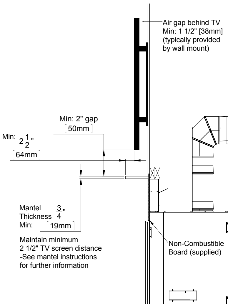
Figure 57: Minimum TV Install
