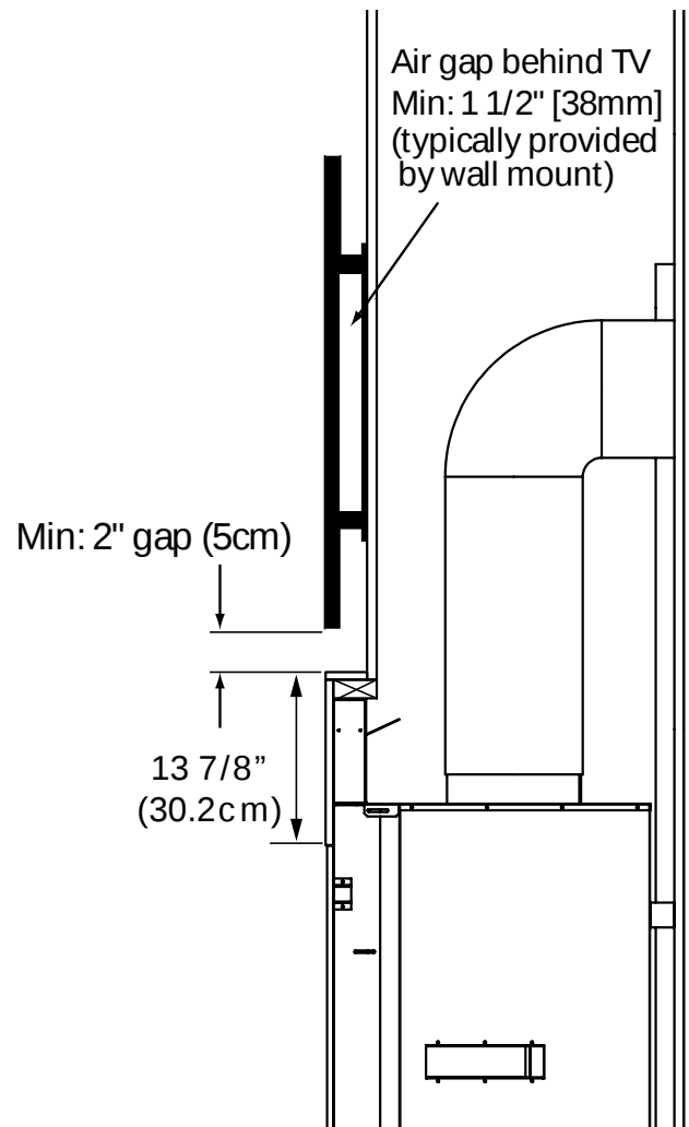
Figure 58: Recess Minimum TV Install
