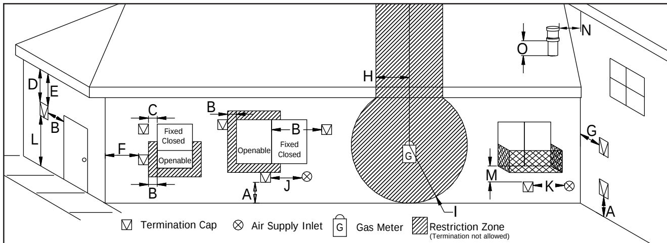
Figure 59: Vent Termination Restrictions, refer to Table 2
