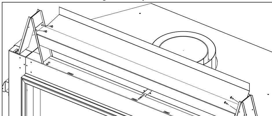
Figure 30: Top Standoff Support Install
