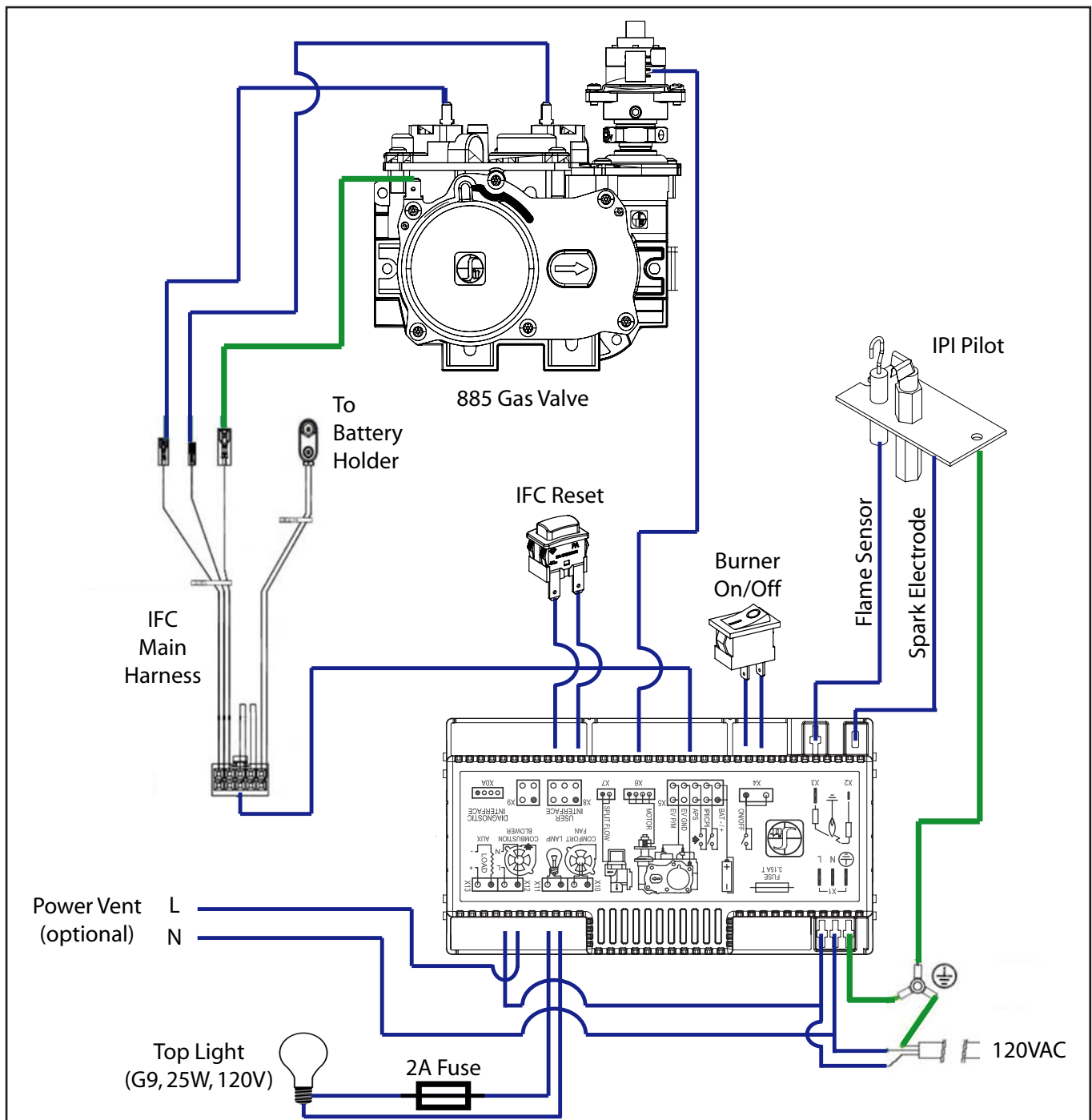
Figure 74: Wiring Diagram
