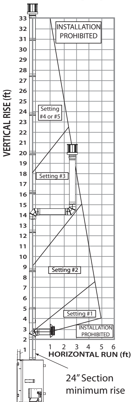
Figure 65: 8" x 11" NG Vent Graph
