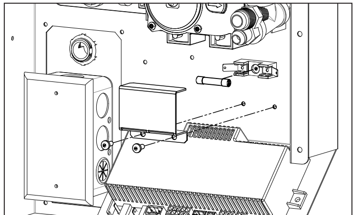
Figure 20: Fuse Removal
