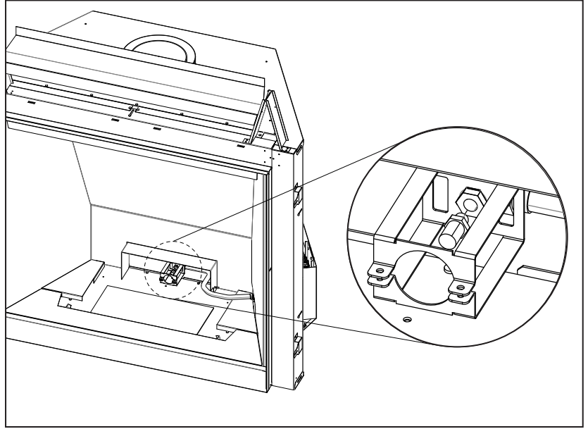
Figure 25: Orifice Location
