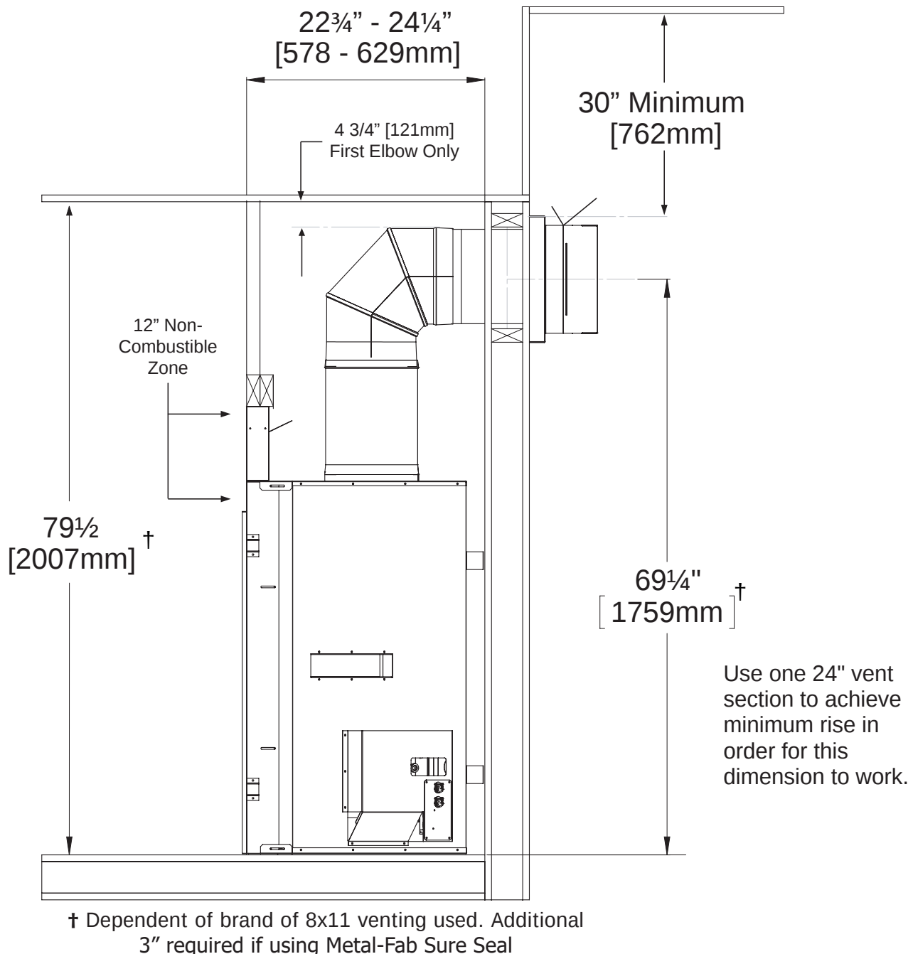
Figure 55: Minimum Vent - 8x11
