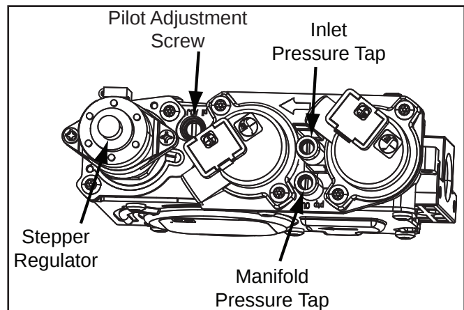
Figure 74: Fully Labeled Gas Valve.
