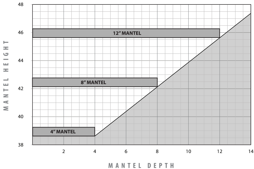
Figure 53: Mantel Clearances - Non CSS
