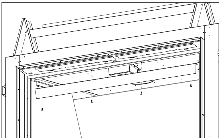
Figure 76: Light Deflector Removal
