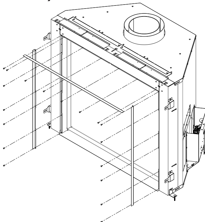
Figure 34: Finishing Edge Removal/ Installation
