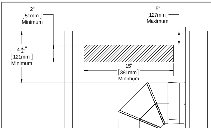
Figure 49: Side Discharge
