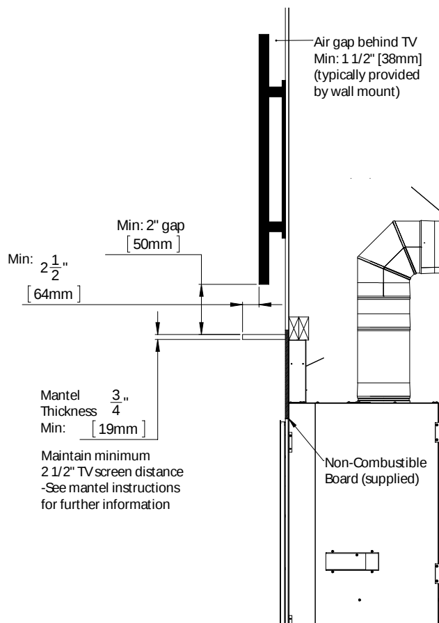
Figure 58: Minimum TV Install
