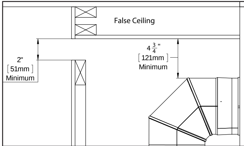
Figure 43: False Ceiling
