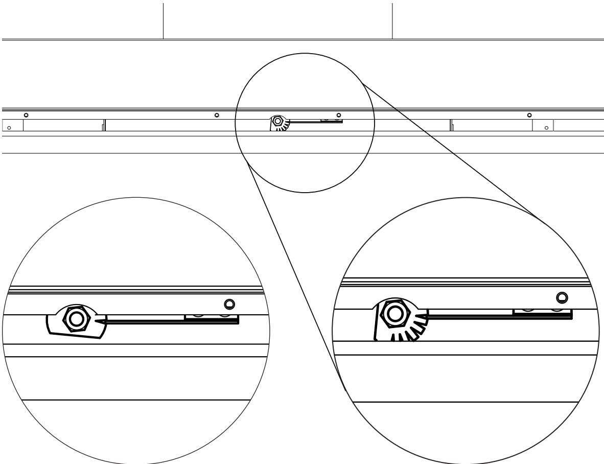
Figure 67: Restrictor Setting 6
