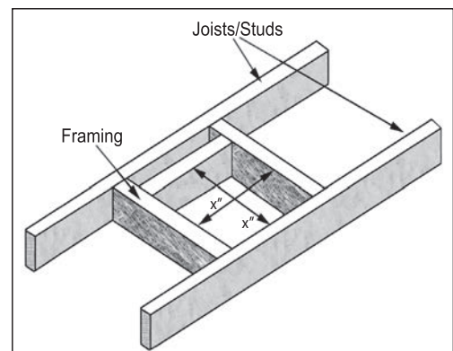
Figure 61: Thimble Framing
