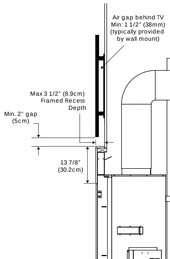
Figure 59: Recess Minimum TV Install
