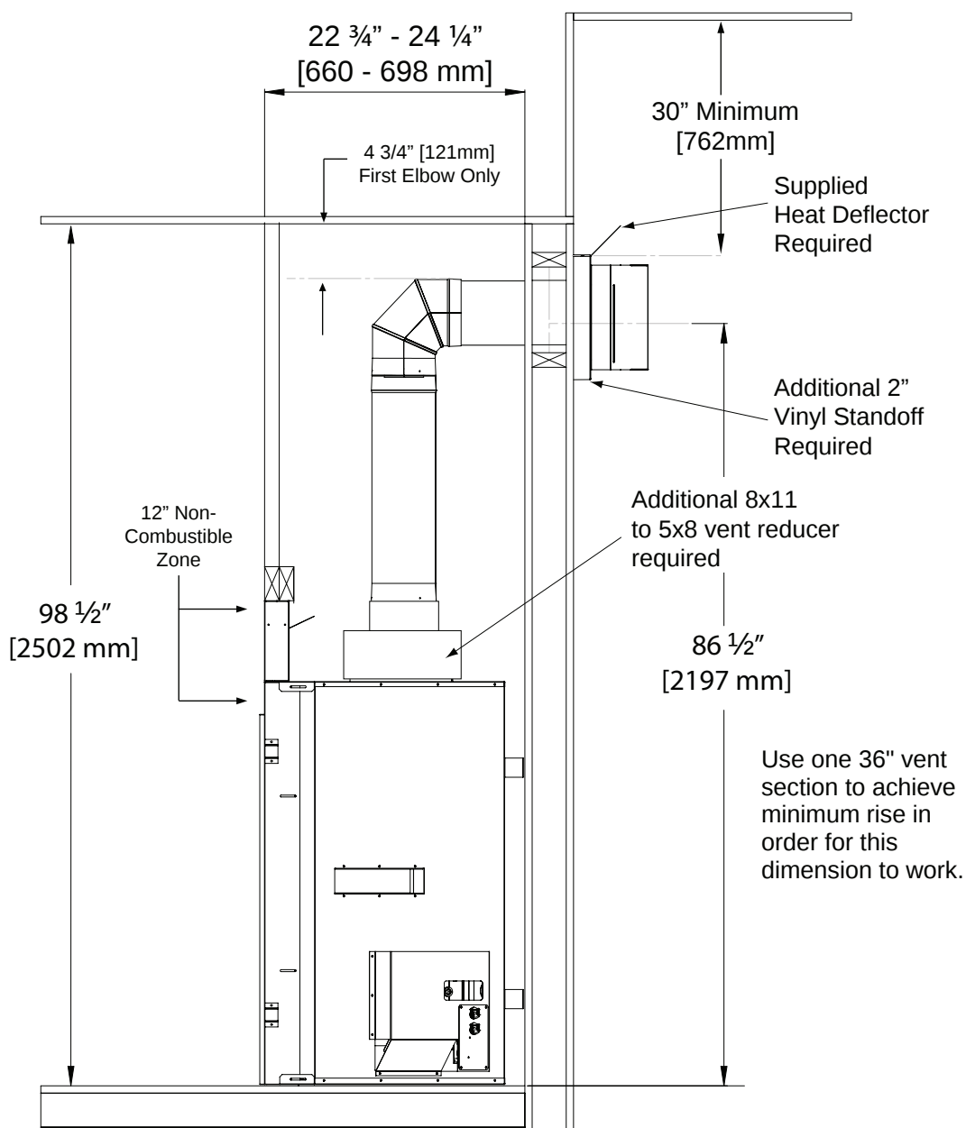
Figure 56: Minimum Vent - 5x8
