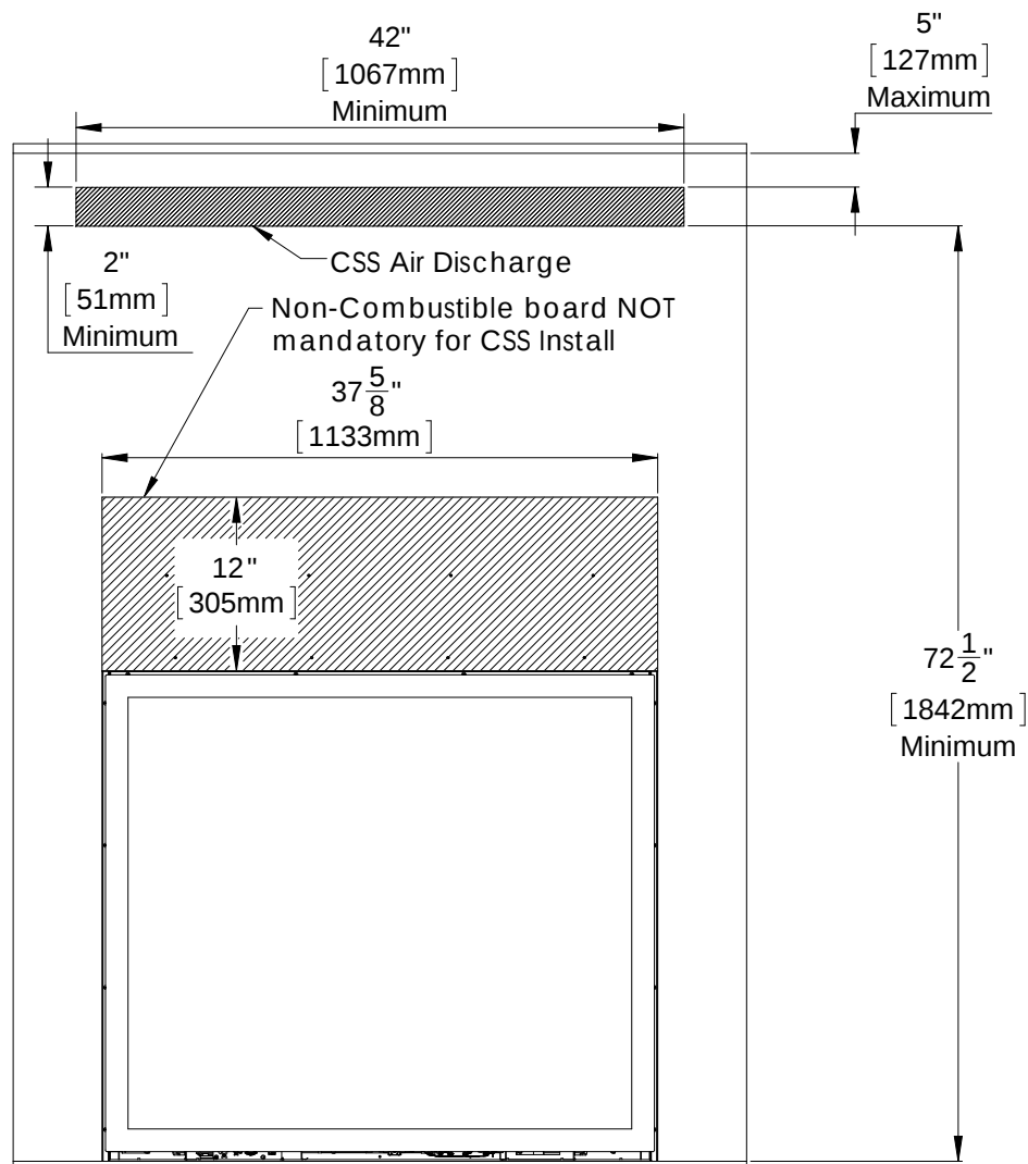
Figure 52: Typical Facing Layout
