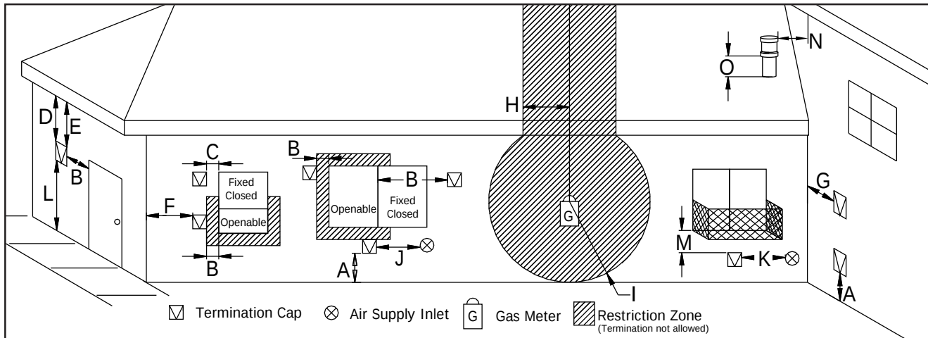
Figure 55: Vent Termination Restrictions, refer to Table 2
