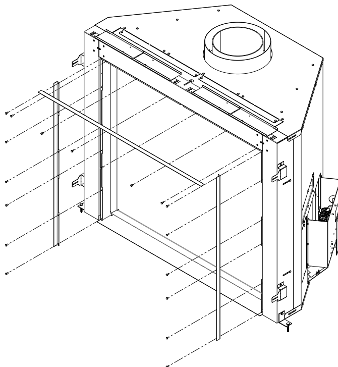
Figure 29: Finishing Edge Removal/ Installation
