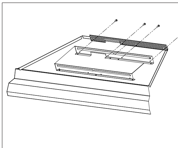
Figure 73: Remove Rear Mesh strip from underneath the porcelain tray by undoing the 4 T20 screws. DO NOT Remove the Front Mesh Strip.
