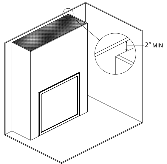
Figure 41: Open Chase Iso View
