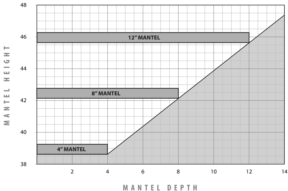
Figure 48: Mantel Clearances - Non CSS
