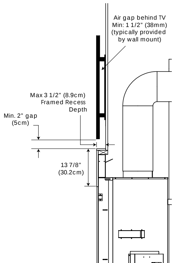
Figure 54: Recess Minimum TV Install
