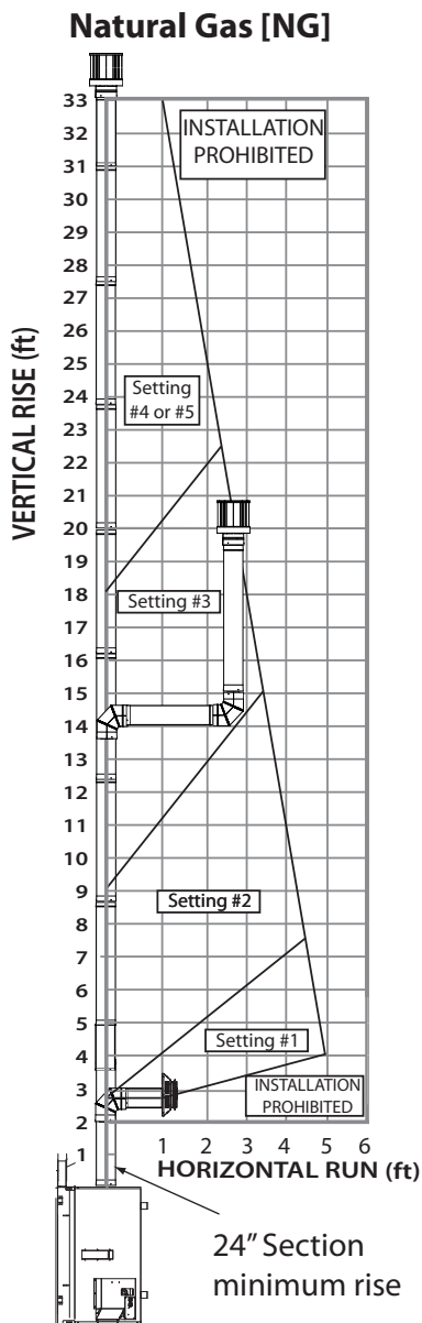
Figure 60: 8" x 11" NG Vent Graph
