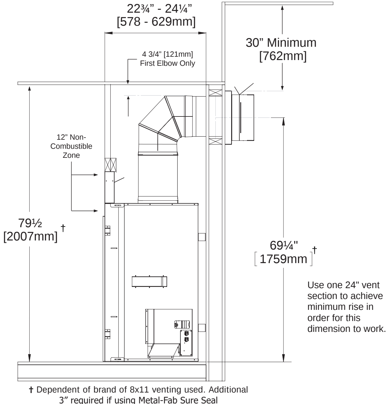
Figure 50: Minimum Vent - 8x11
