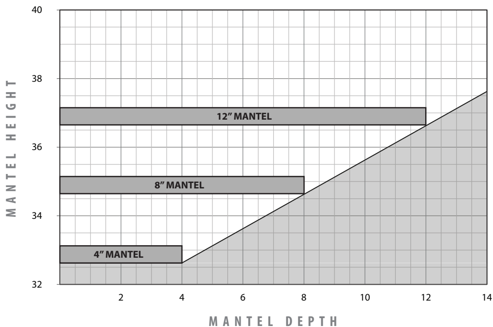
Figure 49: Mantel Clearances - CSS Activated
