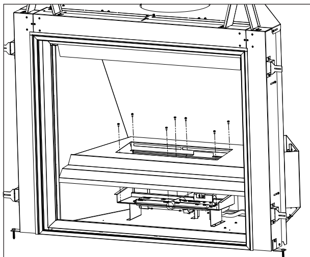
Figure 72: Log Set Remove the Porcelain Tray by removing the seven (7) R20 screws around the board of the burner recess.
