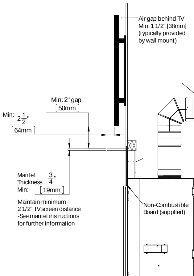
Figure 53: Minimum TV Install
