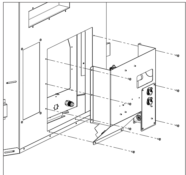
Figure 12: Component Backpack Removal
