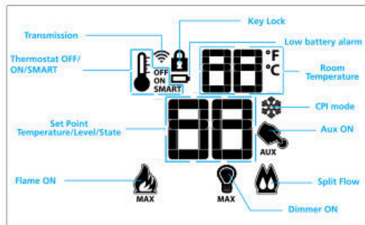
Figure 2: Transmitter LCD Display
