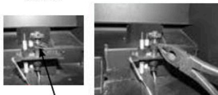
Pilot retainer clip
