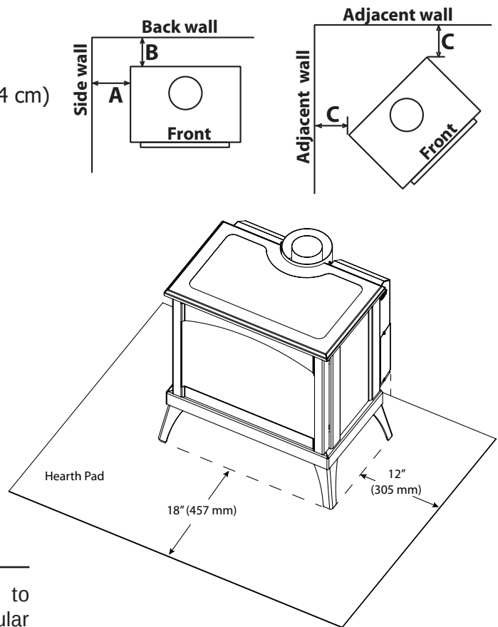
Figure 17: Required Floor Protection Size (vinyl flooring only)
