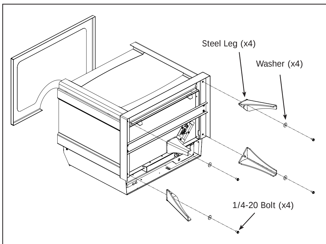
Figure 16: Leg Assembly
