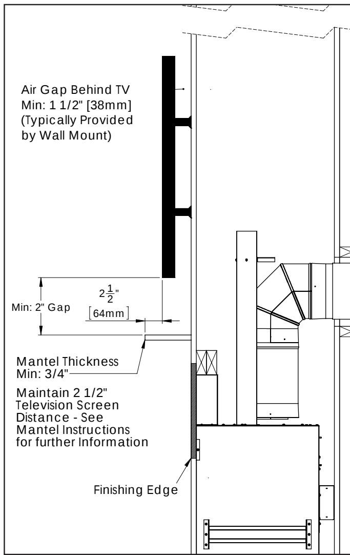
Figure 54: Minimum TV Install Clearances
