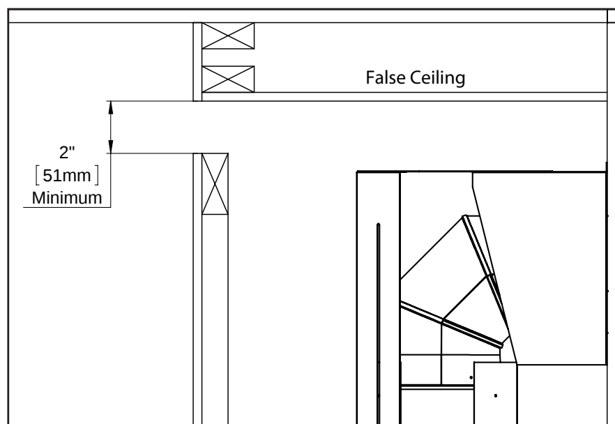
Figure 36: False Ceiling
