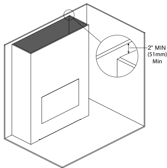
Figure 39: Open Chase Iso View
