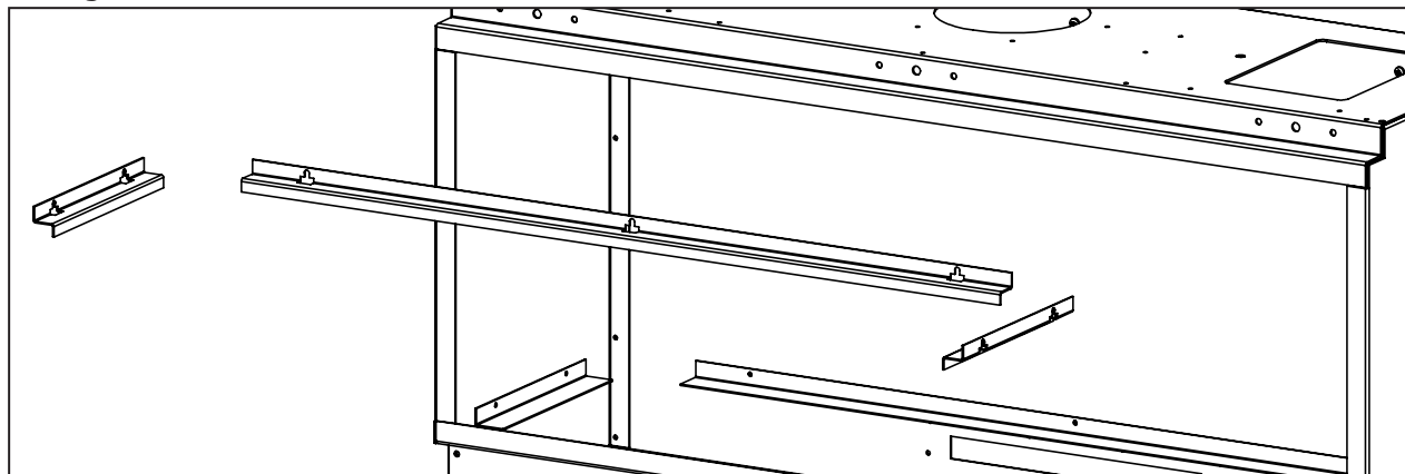
Figure 73: Panel Installation
