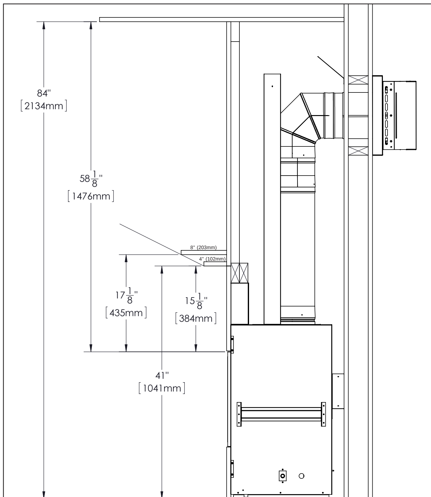
Figure 47: Install Dimensions with Mantel
