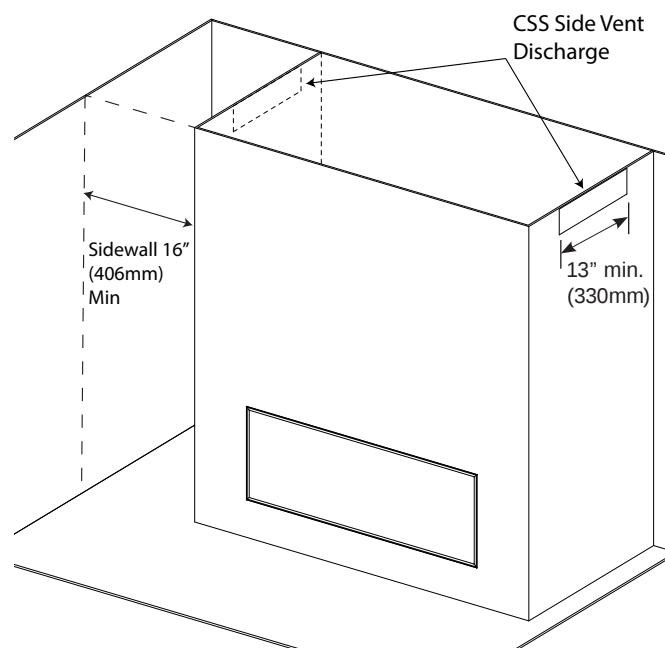
Figure 35: CSS Side Vent
