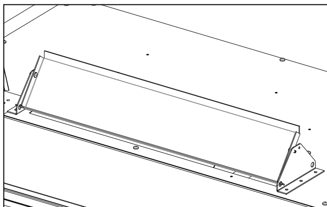
Figure 26: CSS flaps - open
