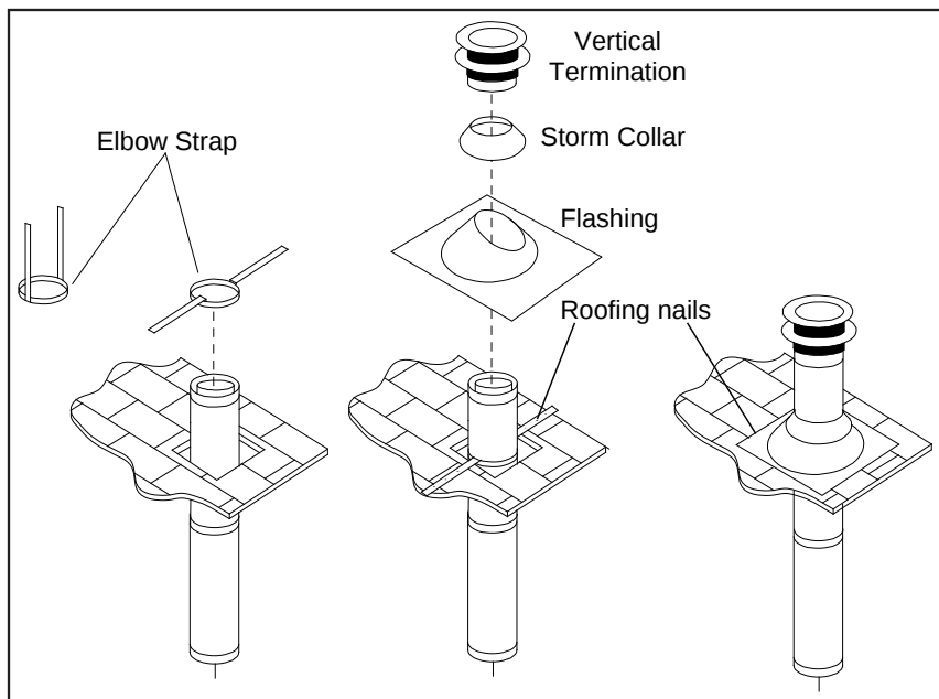
Figure 63: Vertical Vent Termination
