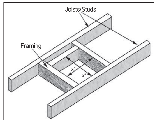
Figure 57: Vent Framing For Wall or Ceiling
