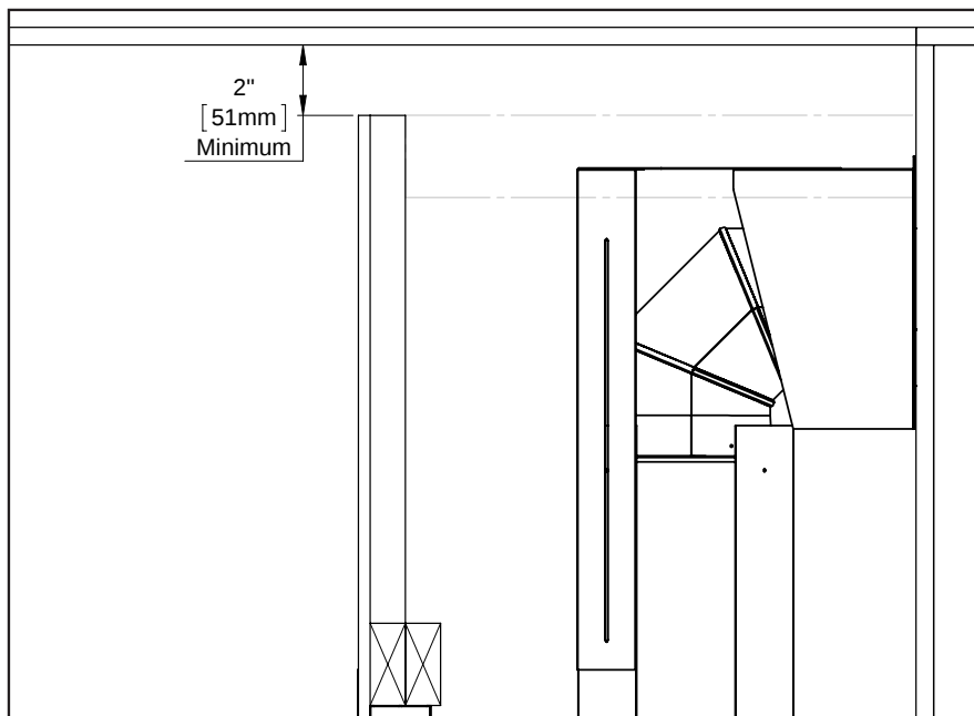
Figure 38: Open Chase
