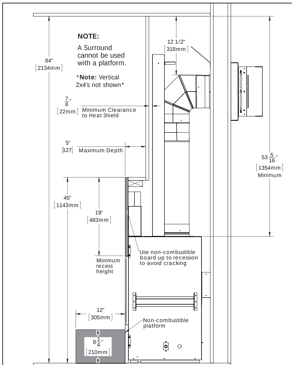
Figure 49: Install Dimensions with Platform
